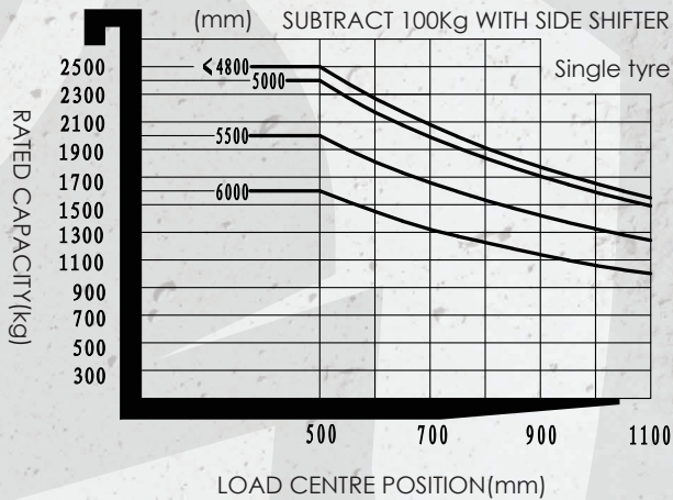
RATED CAPACITIES AND LOAD CENTRES GRAPH
